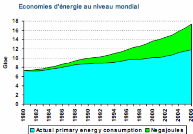
Figure 2.5: Energy savings from energy intensity decrease at world level
